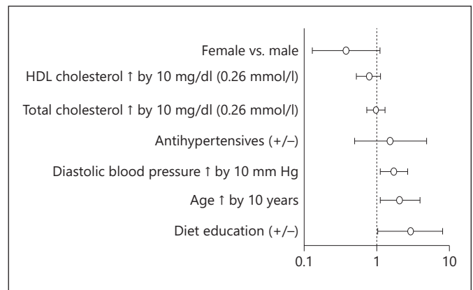
Fig. 7-4. Hazard ratios for acute myocardial infarction (AMI), including suspected cases, and sudden death: area-matched control study for J-LIT [8]. A total of 4,918 participants aged 35–70 years with high cholesterol levels (220–299 mg/dl, 5.69–7.75 mmol/l) were followed for 6 years. In a multivariate model, hazard ratios were calculated with adjustment for age, sex, systolic and diastolic blood pressure, and receipt of dietary education. The risk associated with diet education was 2.87 (95% confidence interval, 1.03–7.96): diet education at that time actually increased the risk for AMI. HDL = High density lipoprotein.
