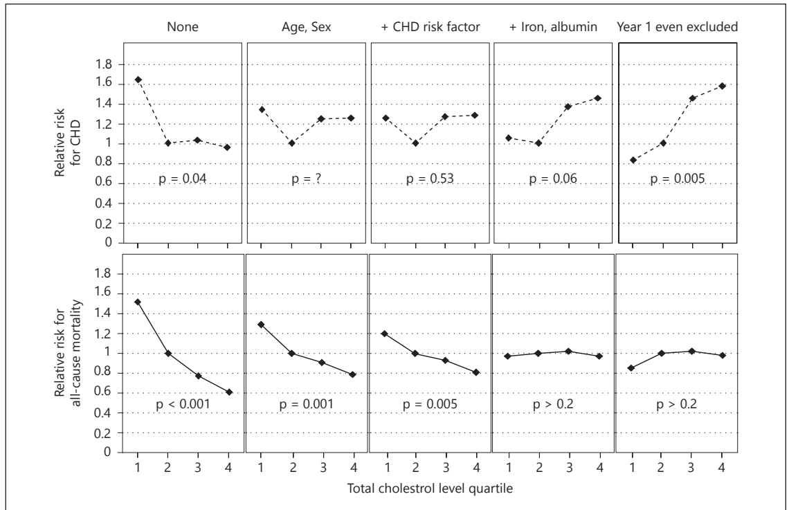
Fig. 5-3. Relative risks for coronary heart disease (CHD) mortality (upper panel) and all-cause mortality (lower panel) according to total cholesterol quartile in elderly persons, as an exemplar of the effects of adjustment factors in analysis [6]. Men and women from three communities in America (n = 4,066, aged >65 years) were followed for 5 years. Baseline measurements were performed in 1988. The correlation of mortality (of CHD in particular) with to-
