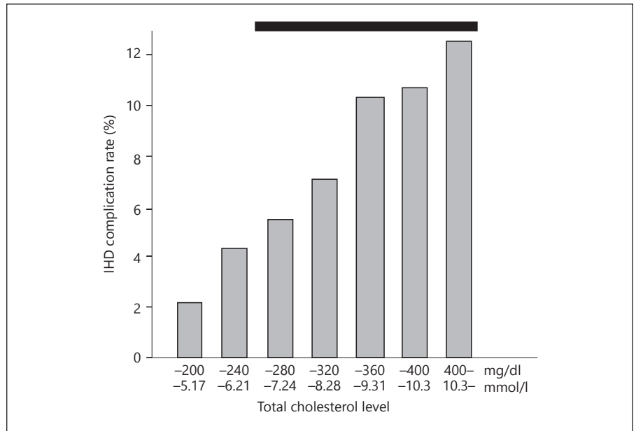
Fig. 3-1. Relationship between total cholesterol level and ischemic heart disease (IHD) complication rate: Research Group for Primary Hyperlipidemia [5]. For 10,313 participants with hyperlipidemia, the IHD complication rate was calculated according to total cholesterol level in this cross-sectional study. There were 1,440 subjects with total cholesterol >6.7 mmol/l (>260 mg/dl), indicated by the black bar. Of them, 388 (27%) were patients with familial hypercholesterolemia (FH). This proportion of FH is more than 130 times higher than that in the general Japanese population. The figure shows that it is highly likely that the proportion of FH cases is increasing along with total cholesterol values. The number of subjects allocated to each column is not available.
