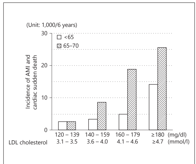
Fig. 7-3. Rough reproduction of the important part of a cholesterol campaign brochure published by Daiichi-Sankyo Company, Ltd. The original of this figure appeared in a sales promotion leaflet for pravastatin, a statin produced by Daiichi-Sankyo Company, Ltd. The original data come from one of the J-LIT Study reports (figure 1, panels A and B) [7]. However, note the start point of the X-axis is 120–139 mg/dl (3.1–3.5 mmol/l): the left part of both original panels was deleted in the figure shown here, because the major coronary events were slightly increased in the LDL cholesterol ranges <100 mg/dl (0.26 mmol/l) and 100–119 (2.6–3.0) in the elderly group aged 65–70 years. The all-cause mortality is not shown in the leaflet either. See the text and table 7-B for more problems with this leaflet. The important point for us here is that the Chief Editor of the 2012 JAS Guidelines supervised the making of this leaflet. AMI = Acute myocardial infarction; LDL = low density lipoprotein.
