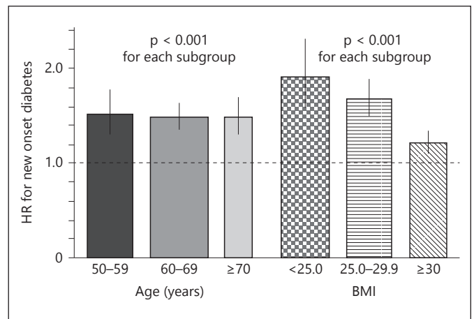
Fig. 9-1. Association between diabetes risk and statin use status at baseline, according to age and body mass index (BMI) subgroups in women: Women’s Health Initiative [7]. A total of 153,840 postmenopausal women without diabetes aged 50–79 years were followed for a mean period of 6.5 years. Statin use at baseline was associated with incidence of new onset diabetes (multivariate adjusted hazard ratio: 1.48, 1.38–1.59). Adjusted for age, race/ethnicity, education, cigarette smoking, BMI, physical activity, alcohol intake, energy intake, family history of diabetes mellitus, hormone therapy, study arm (42% of participants were enrolled in clinical trials), and self-report of cardiovascular disease at baseline. Age and BMI were excluded in models for the age and BMI subgroups, respectively. The width of each column is proportional to the number of subgroup participants at baseline. HR = Hazard ratio.
